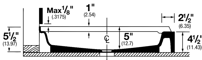
Sectional View
